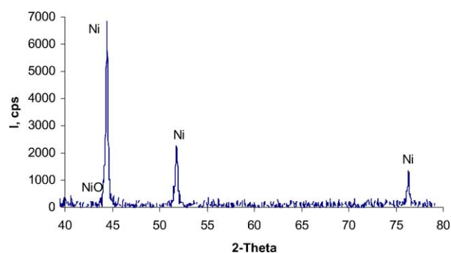
Fig. 2. XRD pattern of Ni nanopowder.
