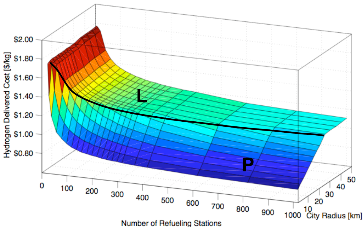
Figure 11 Hydrogen distribution cost [$ /kg] to a network of refueling stations (1800 kg/day capacity) as a function of the number of refueling stations in the network and the radius of the circular city.
