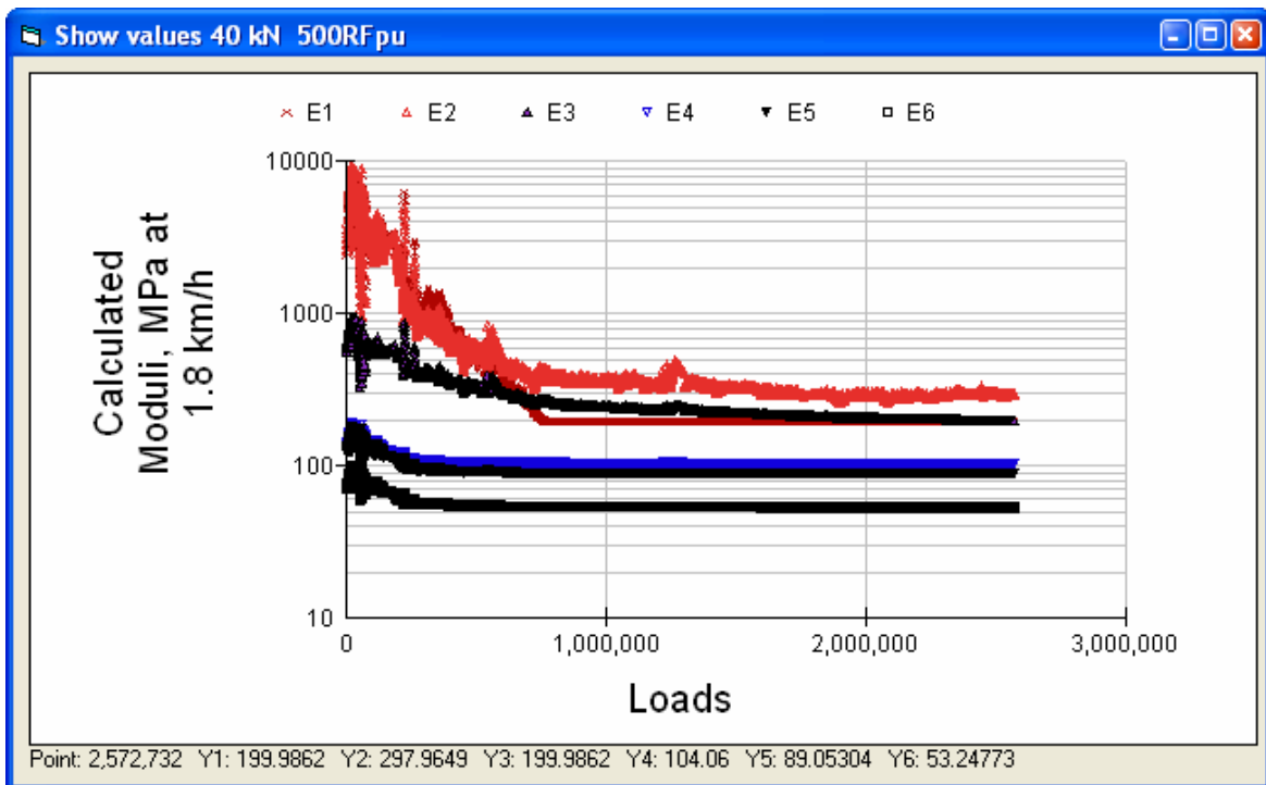
Figure 52. Section 500RF calculated moduli at 40 kN and actual temperature.
