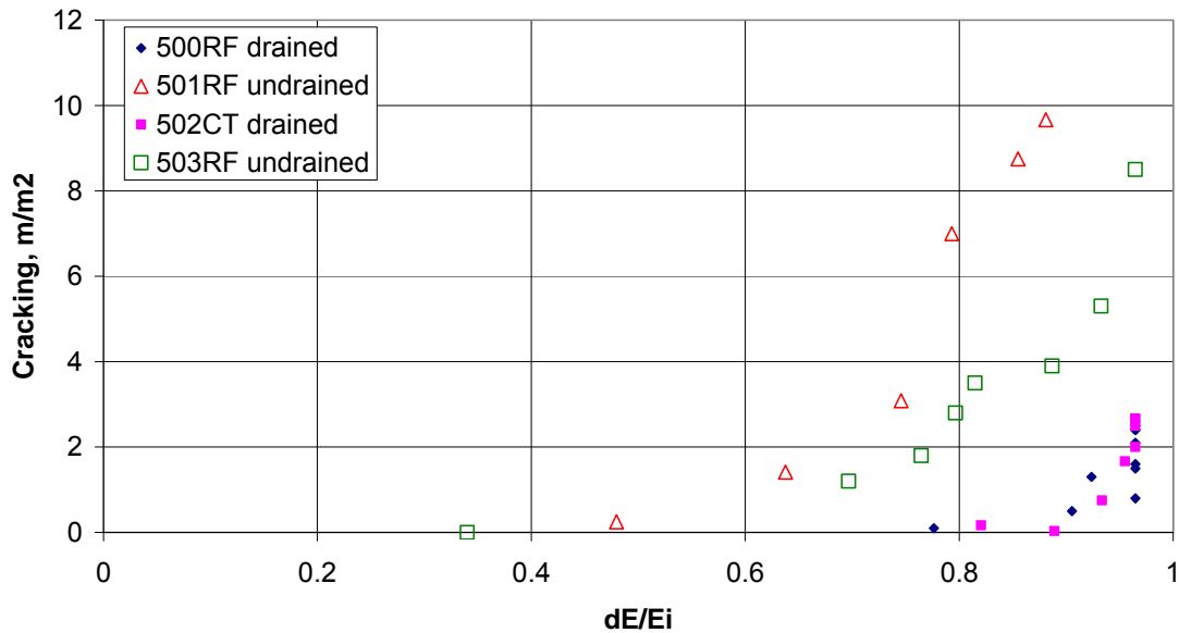
Visual cracking versus decrease in modulus
