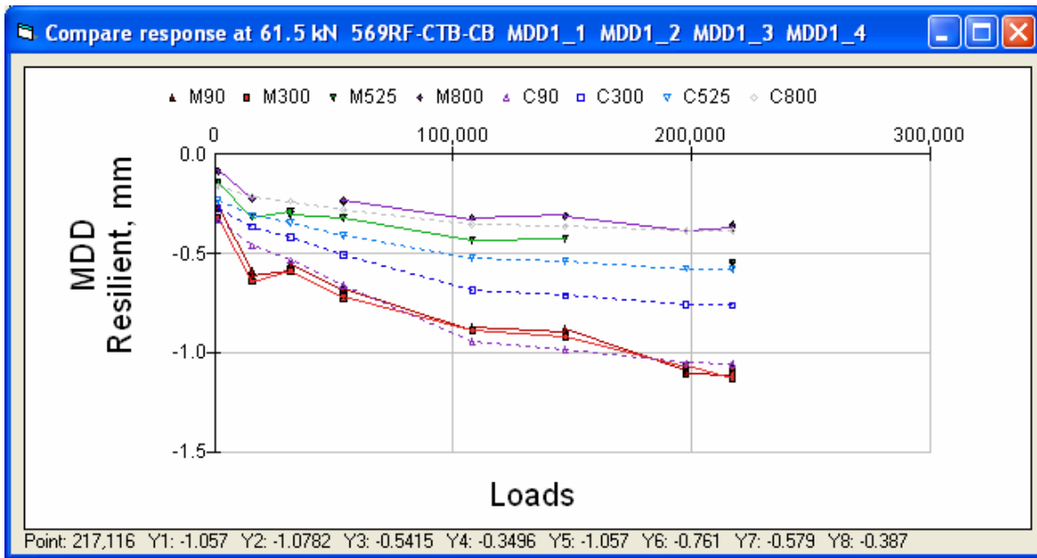
Figure 280. Section 569RF MDD resilient deflections.
