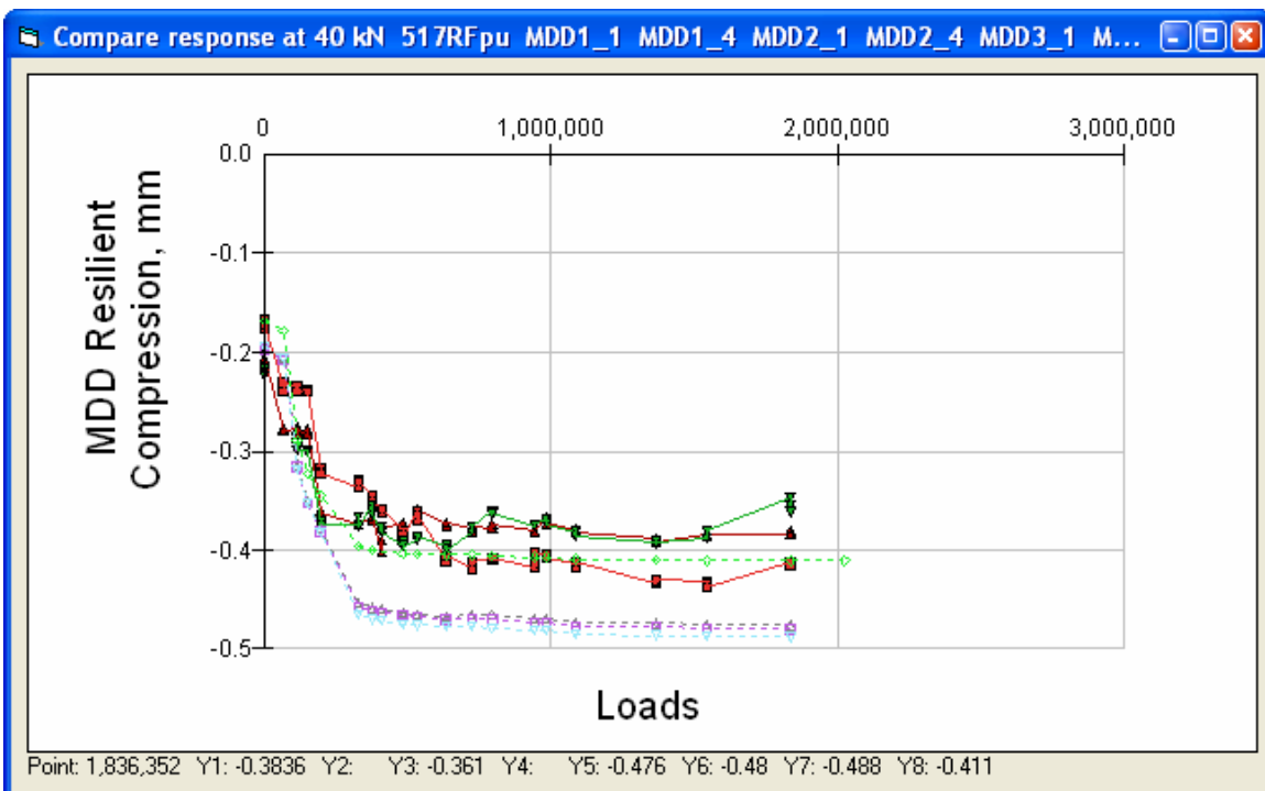
Figure 82. Section 517RF 40 kN compression of pavement layers.
