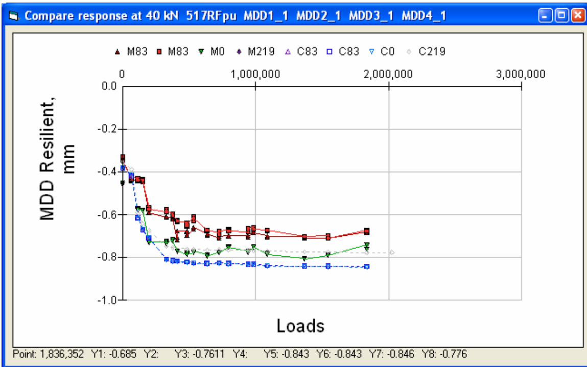
Figure 81. Section 517RF 40 kN deflection of top modules.
