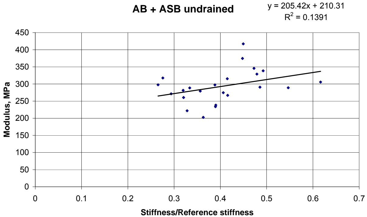
Figure 17. Modulus of Layer 2 as a function of the stiffness of the asphalt layers, for the undrained sections.
