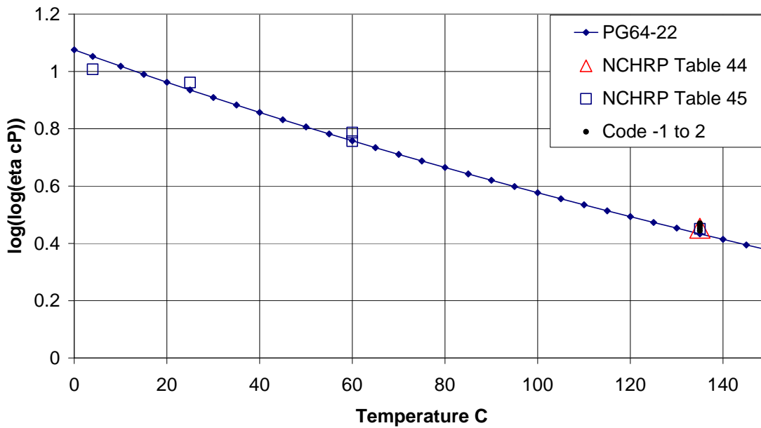
Figure 34. Lay-down viscosity, in cPoise, PG64-22 and measured viscosity, versus temperature. (Note: NCHRP refers to viscosity values from NCHRP Report 455, Reference 3.)
