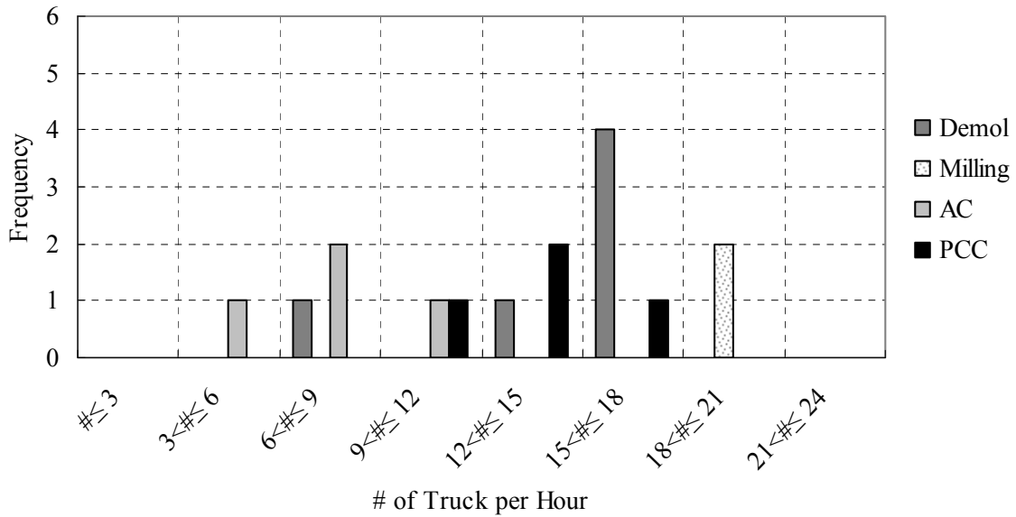
Figure 21: Truck-load frequency during Stage 3C (fourth weekend closure, NB I-15, 44-hrs).
