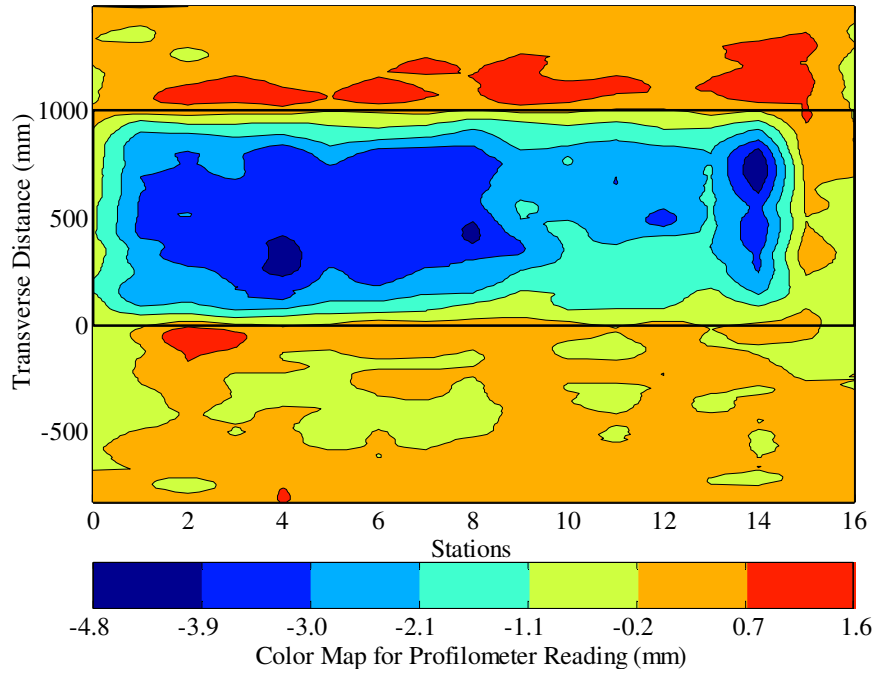
Figure 3.27: Contour plot of permanent deformation after 760,000 repetitions.
