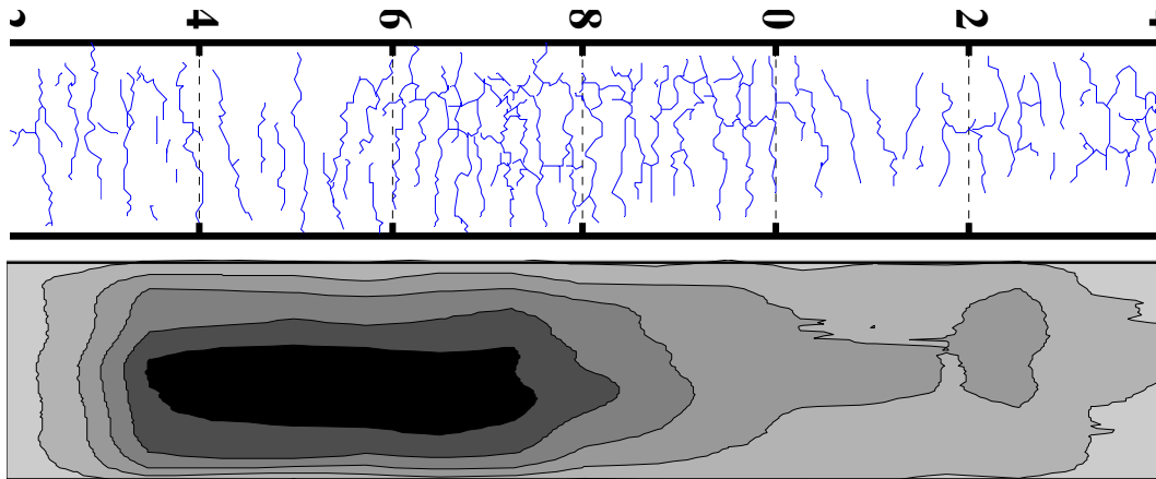
Figure 3.32: Comparison of cracking pattern from Phase 1 and rutting in Phase 2.
