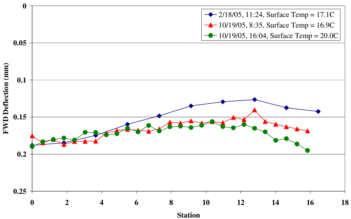
Figure 3.16: Composite pavement stiffness (FWD Sensor 1) outside trafficked area.
