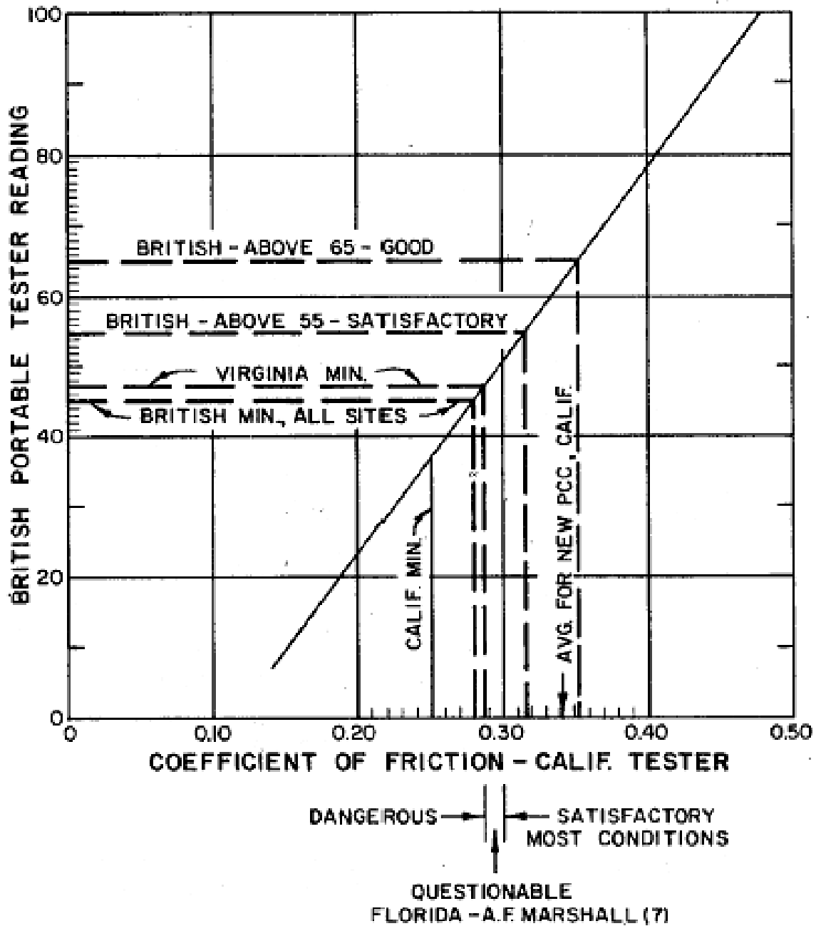
Figure 11: Correlation of California Skid Tester and British Portable Tester. (8)
