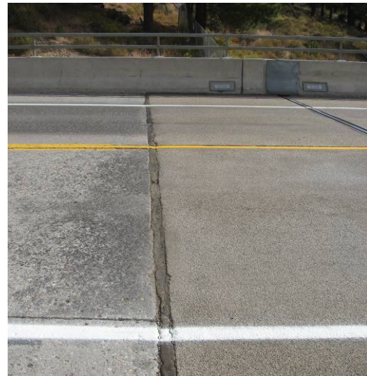
Figure 4.98: Beginning of Section QP-145.1 (right side of photos), Year 1 (left) and Year 2 (right).
