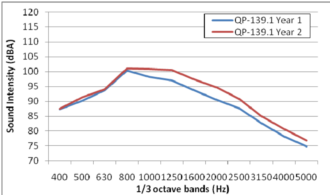
Figure 4.66: OBSI spectra of Section QP-139.1, Year 1 and Year 2.
