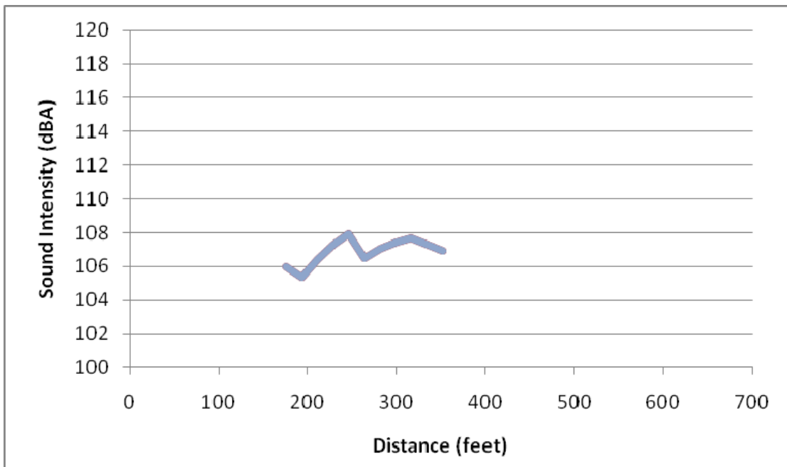
Figure 4.65: OBSI level in 0.2-sec intervals of Section QP-139.1, the bridge only, Year 2, average of three passes.
