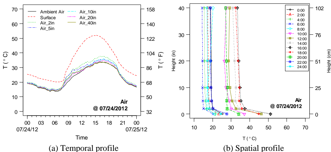
Figure 9.5. Example profiles of near-surface air temperatures on concrete pavement PC1.
