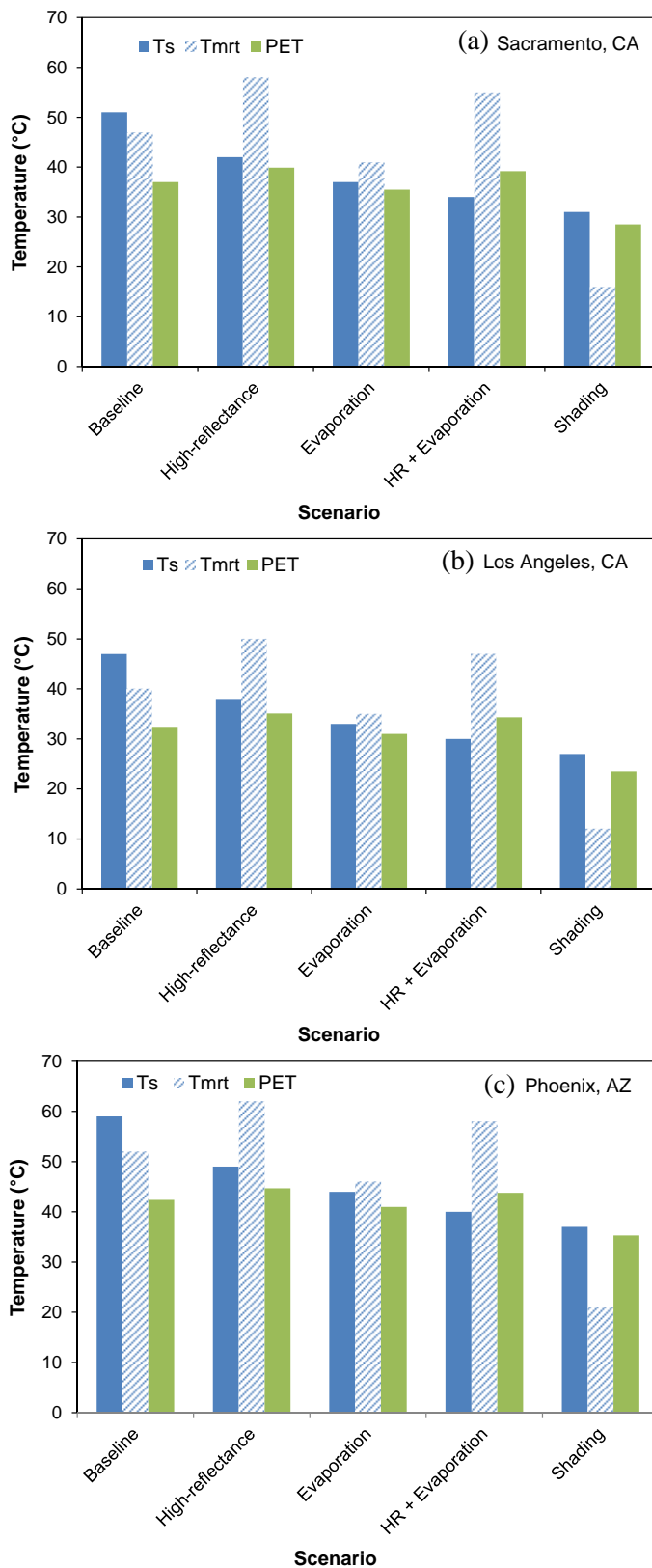
Figure 13.5. Calculated results for different pavement scenarios at three regions: pavement surface temperature T_s , Mean Radiant Temperature T_{mrt} , and PET (summer).
