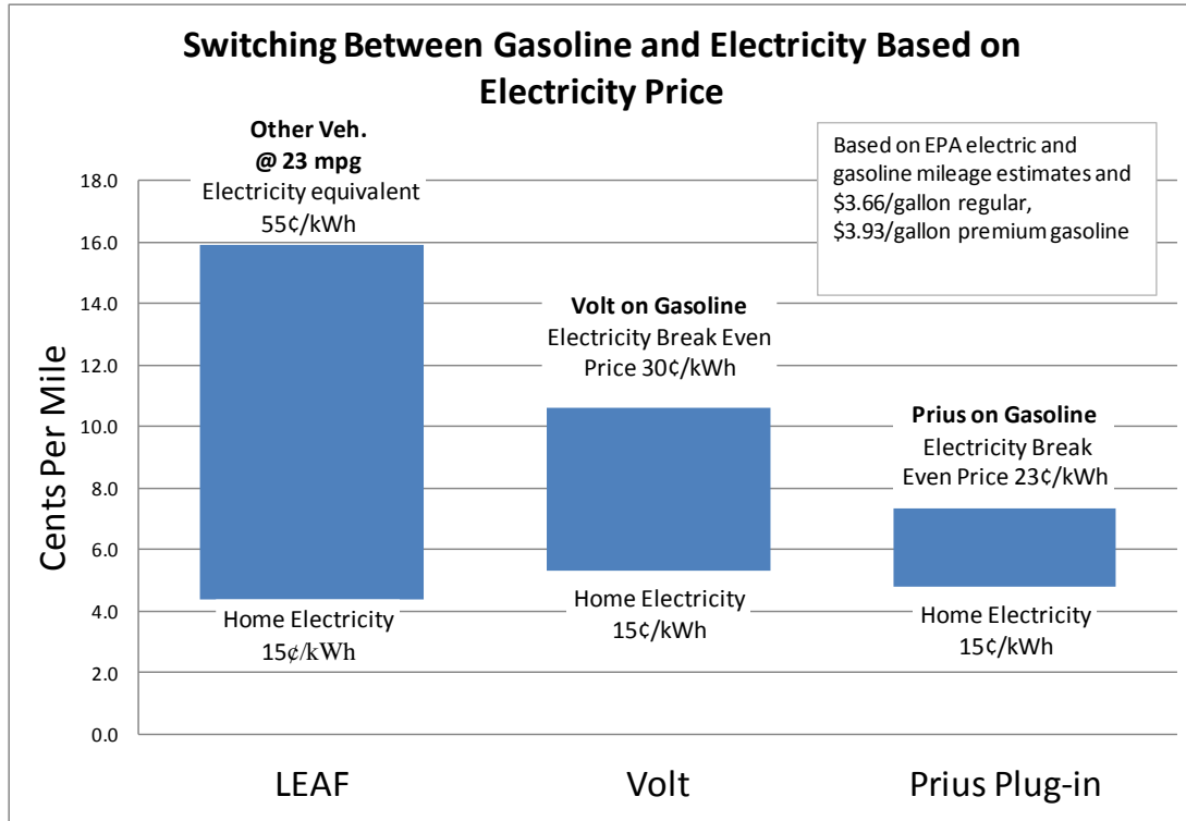
FIGURE 3: Electricity breakeven price points when arbitraging electricity against gasoline.
