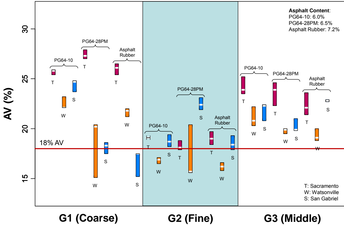
Figure 3.3: Boxplots of air-void content versus gradation, binder, and aggregate type, respectively.
