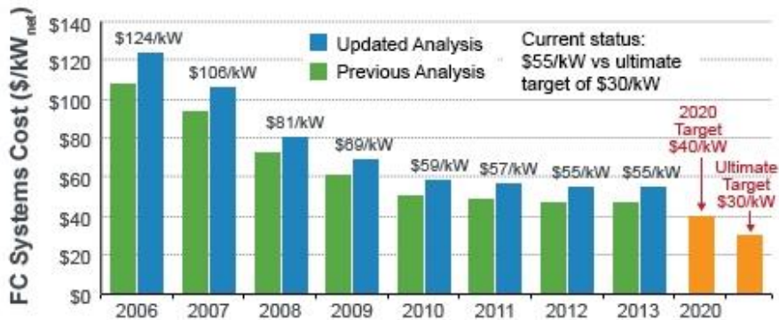
Figure 3. Estimated mass-produced cost of automotive fuel cell systems, and targets for 2020 and long term. Source: US Department of Energy, http://energy.gov/eere/fuelcells/achievements-and-progress , 2014.
