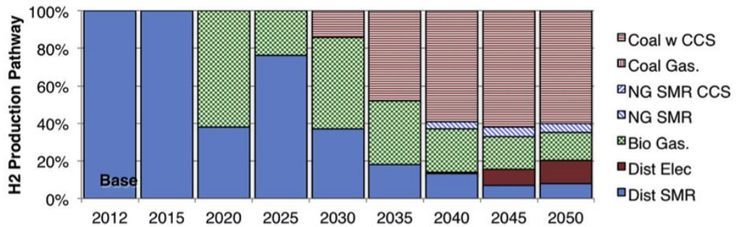
Figure 19. H2TIMES Base case hydrogen production choices aggregated across all regions
