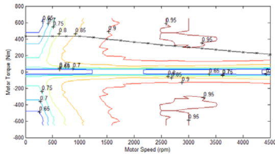
Figure 6: Traction motor efficiency map
