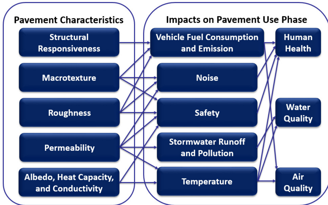
Figure 4-11. Pavement characteristics and influences on use-stage objectives (Van Dam et al. 2015).
