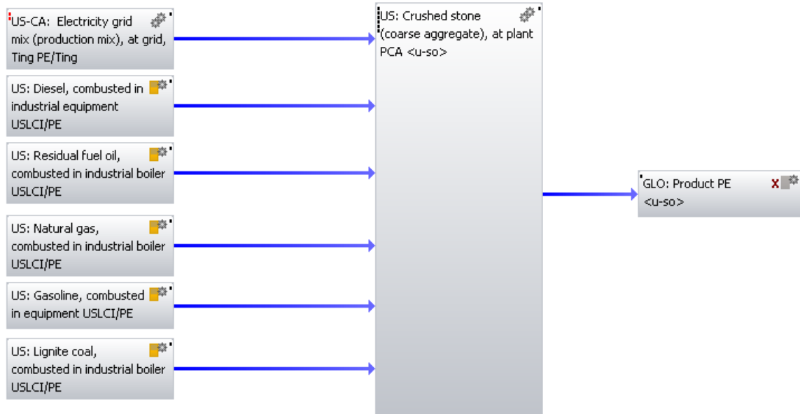
Figure 6-7. GaBi model developed to calculate LCI and LCIA of crushed aggregate production in California (thinkstep 2015).
