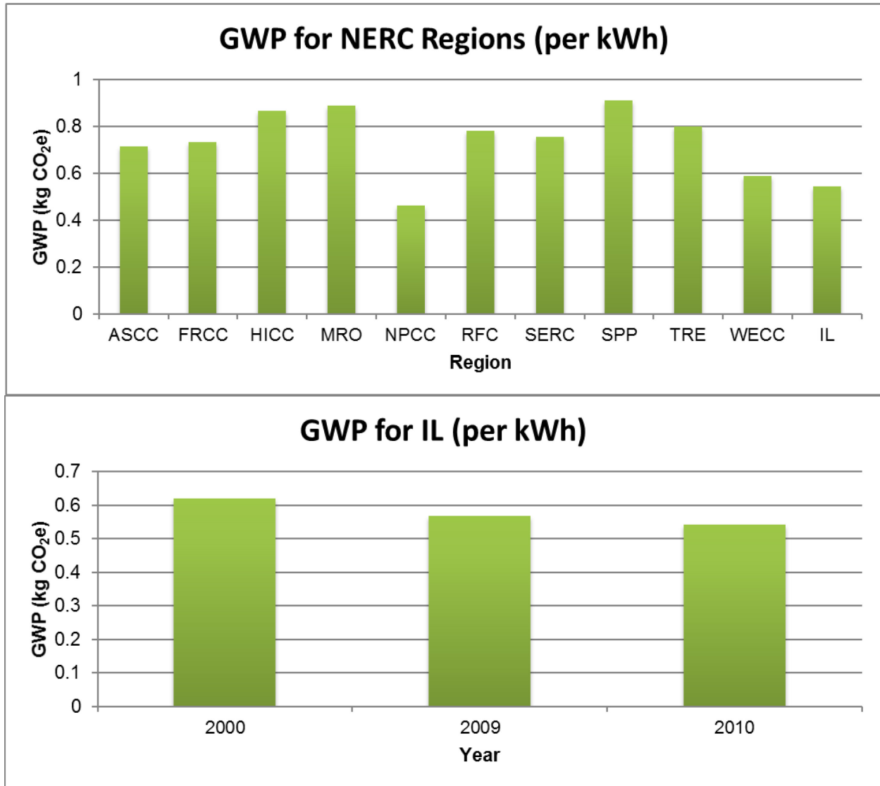
Figure 4-20. Regional and temporal variations in power production in different regions of the U.S. (data source: EPA 2015).
