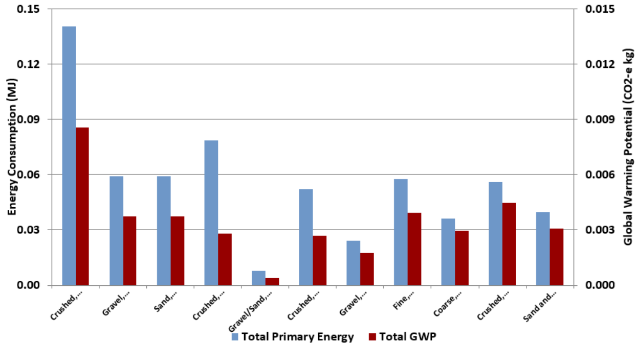
Figure 4-17. Primary energy and global-warming potential from aggregate production per kg, at quarry (after Wang et al. 2012).
