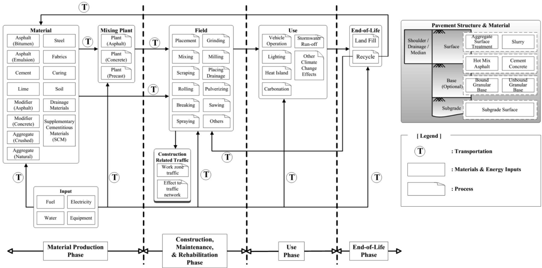
Figure 3-7. UCPRC LCA framework showing major life-cycle stages of a pavement (Harvey et al. 2011).
