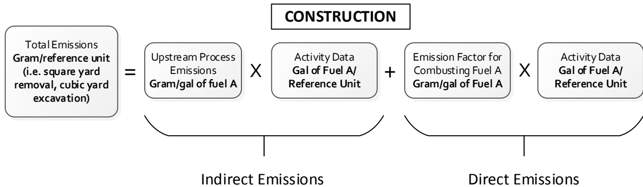
Figure 4-10. Calculation of construction-related emissions.
