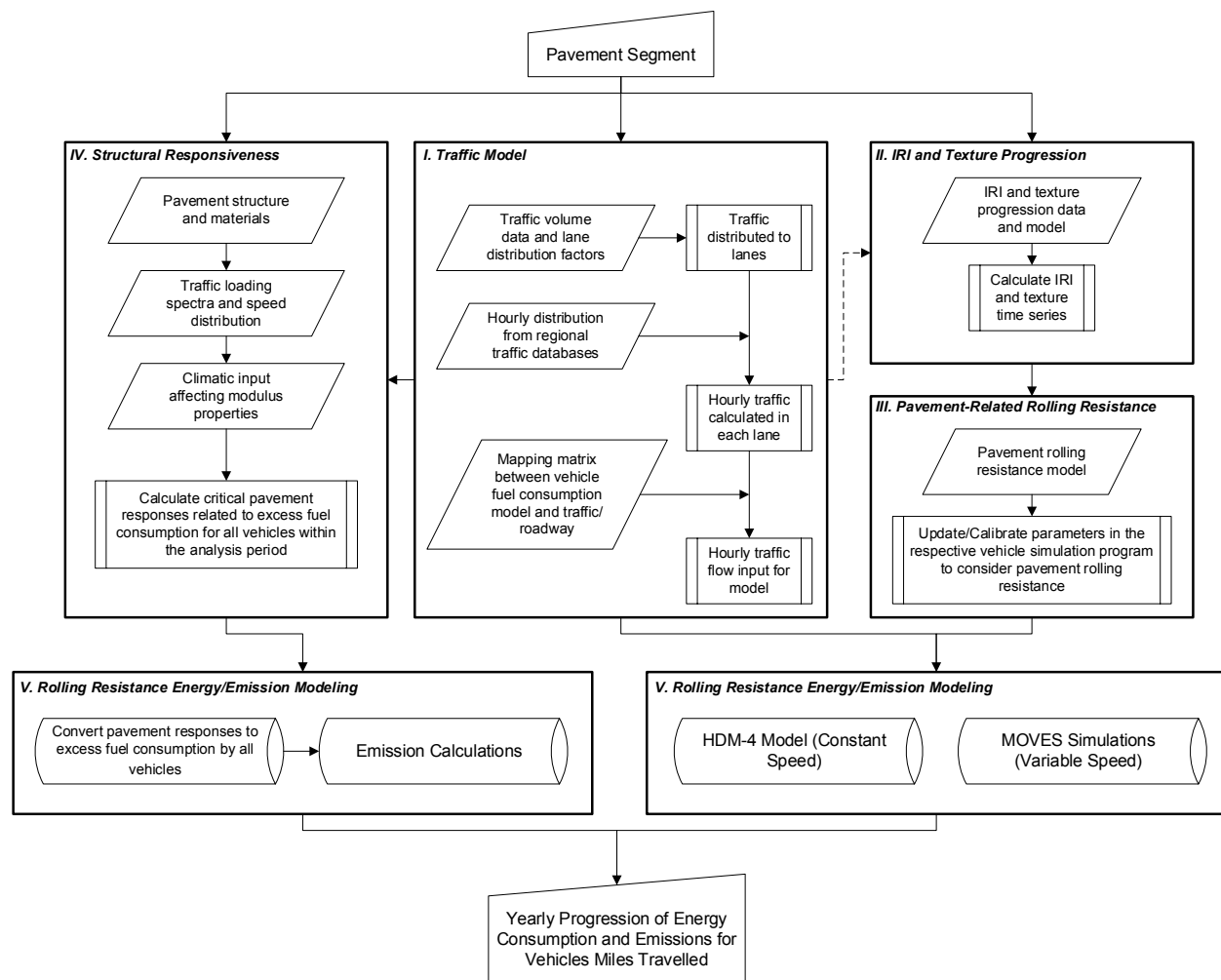
Figure 4-12. Procedures adopted by UCPRC to calculate use-stage inventory input-outputs for vehicle-pavement interaction (adapted from Wang et al. 2012).
