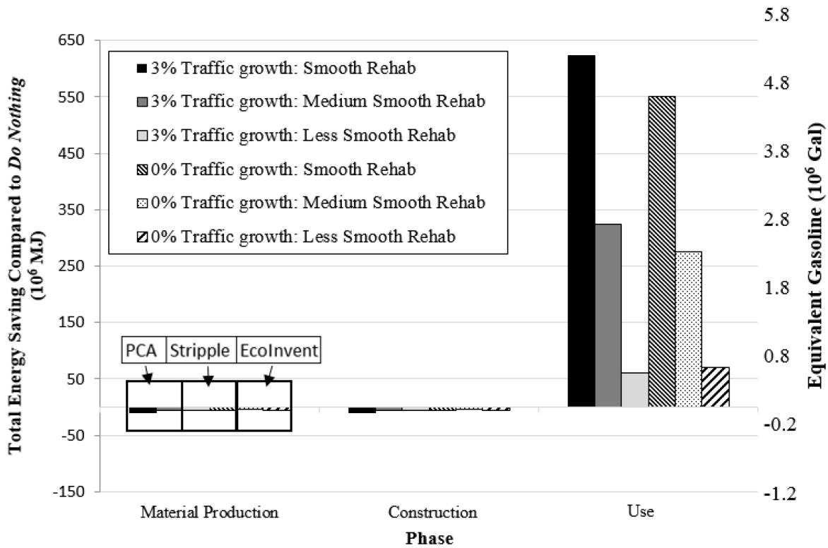
Figure 6-4. Analysis period energy savings compared to Do Nothing with Type III cement on LA-5 (Wang et al. 2012). (Note: diesel use converted to equivalent gasoline in terms of energy.)
