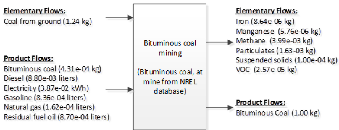
Figure 4-2. An example unit process for coal mining with typical inputs and outputs (NREL 2015).
