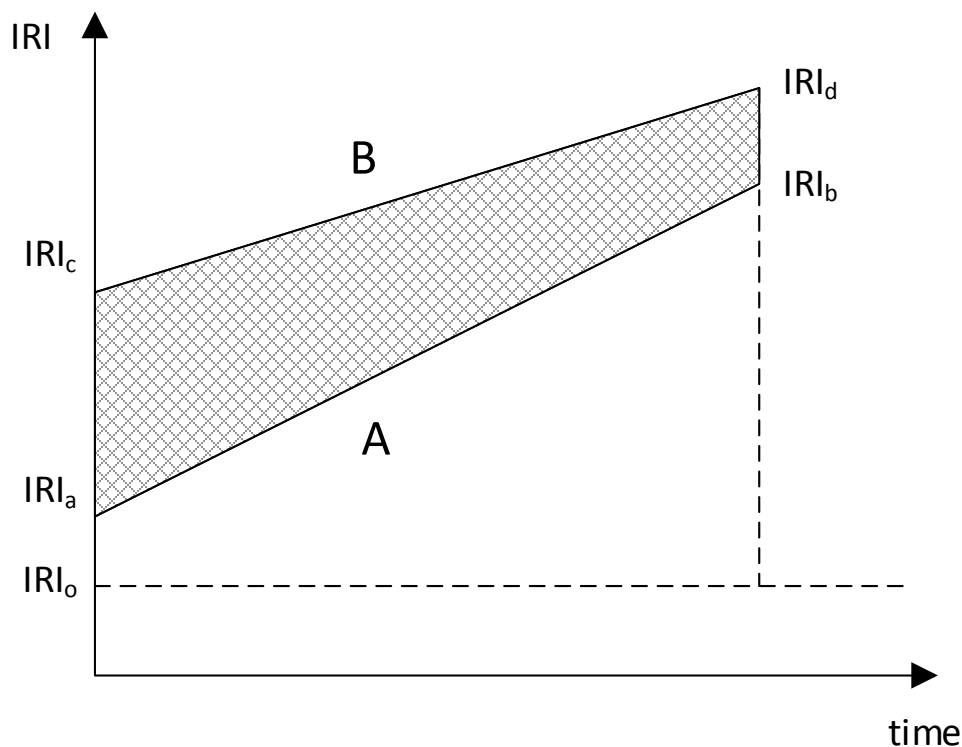
Figure 4-14. IRI progression of two pavement surfaces with the incremental changes illustrated with respect to a reference IRI ( IRI_0 ).
