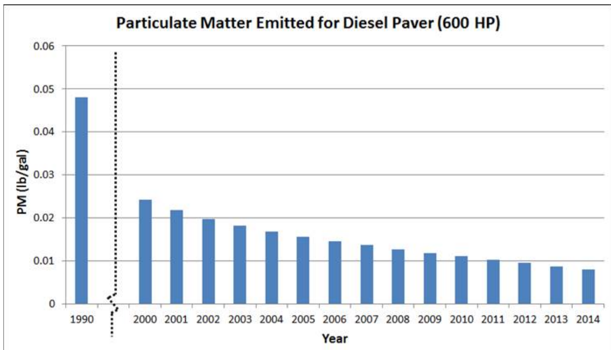
Figure 4-19. Variation of particulate-matter emissions from a diesel paver between 1990-2014 (data source: EPA 2008b).
