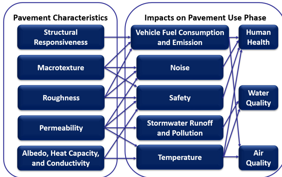
Figure 2-3. Selected pavement characteristics and their impacts on use-phase objectives (Van Dam et al. 2015).
