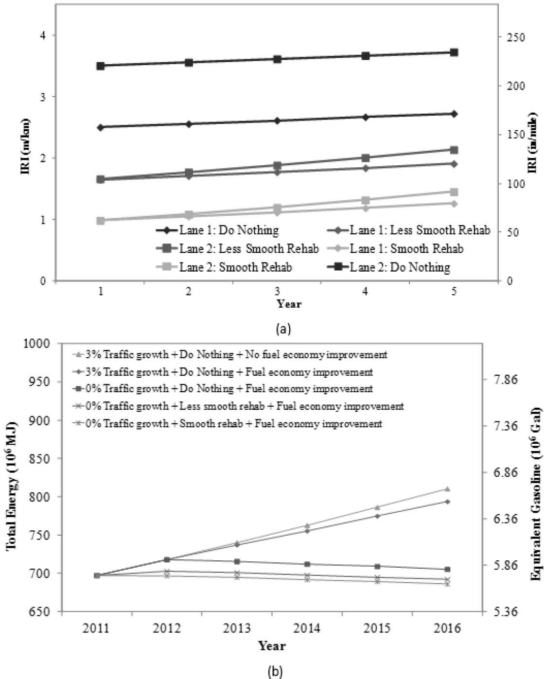
Figure 4-13. (a) IRI progression for various rehabilitation scenarios, (b) Corresponding additional energy consumption for each scenario (Wang et al. 2012).
