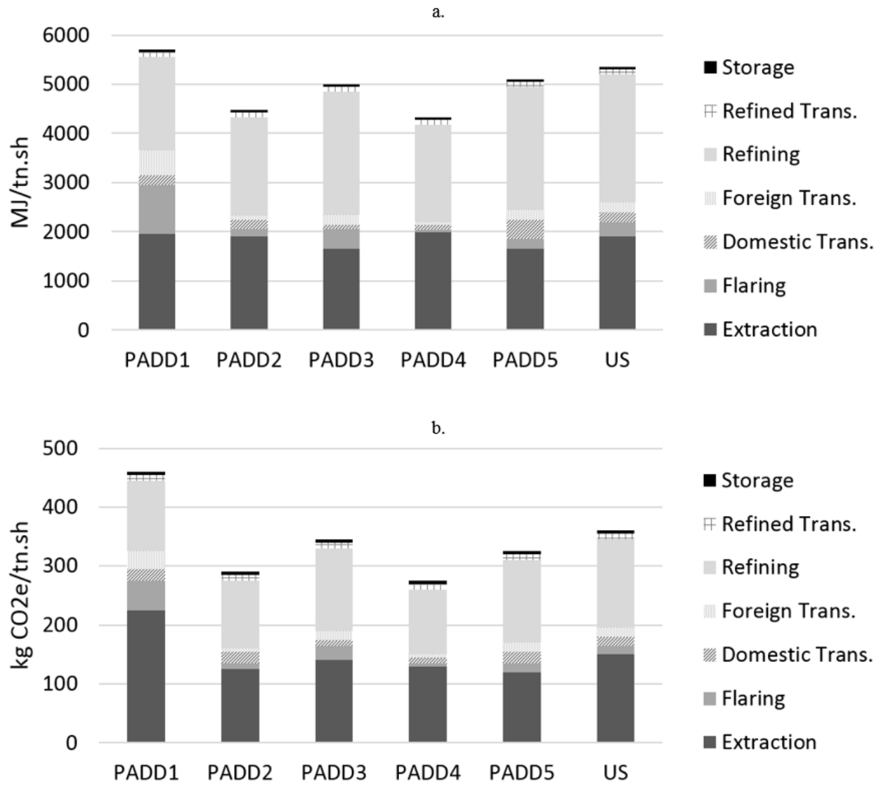
Figure 4-21. Life-cycle results for asphalt-binder production with respect to different regions in the U.S. (Yang 2014).
