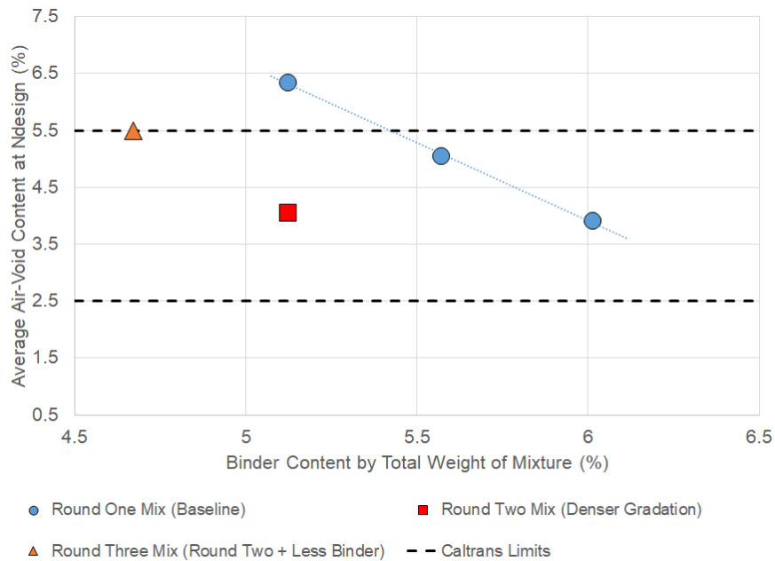
Figure 6.1: Air-void content at Ndesign gyrations for the Round One, Round Two, and Round Three mixes.
