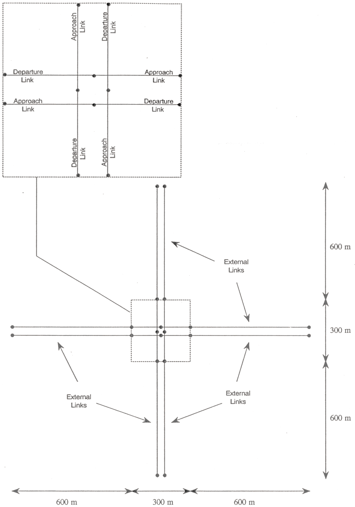
Figure B.2 Link Network for a Single Intersection with no Dedicated Left-Turn Lanes.
